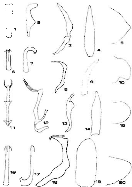
FIGURES 1-20. Figs. 1-5: Gypona scabella (1) aedeagus ventrally, (2) aedeagus laterally, (3) style laterally, (4) plate ventrally, (5) pygofer laterally, apical portion. Figs. 6-10: G. concessa (6) aedeagus ventrally, (7) aedeagus laterally, (8) style laterally, (9) plate laterally, (10) aedeagus laterally, apical portion. Figs. 11-15: G. fulvanota (11) aedeagus ventrally, (12) aedeagus laterally, (13) style laterally, (14) plate ventrally, (15) pygofer laterally, apical portion. Figs. 16-20: G. barda (16) aedeagus ventrally, (17) aedeagus laterally, (18) style laterally, (19) plate ventrally, (20) pygofer laterally, apical portion.
