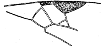
Fig. 5. Microgaster primordialis sp. nov. Part of fore wing.
