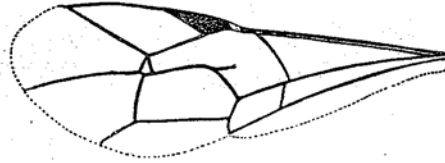
Fig. 4. Pimpla appendigera sp. nov. Fore wing. Dotted lines are restored.
