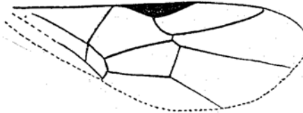
Fig. 2. Accenites defunctus sp. nov. Fore wing. Dotted lines are restored.
