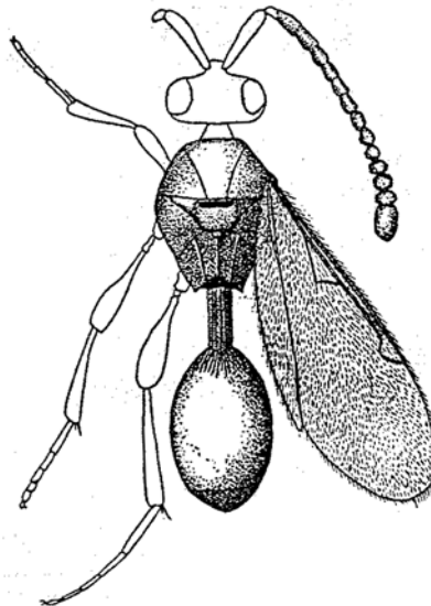
Fig. 6. Pantoclis deperdita sp. nov. Restored parts are unshaded.
